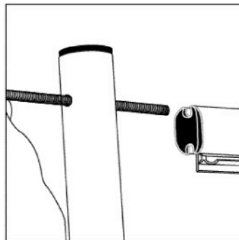
Slide threaded rod through the top hole of one vertical pole and then through top channel of one AnoQuick holder. Note: Picture shows Anogotcha. Assembly is the same.
